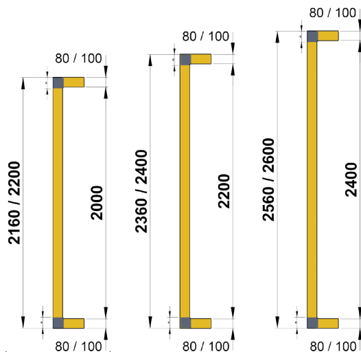
CON suelo panel WITH floor panel
